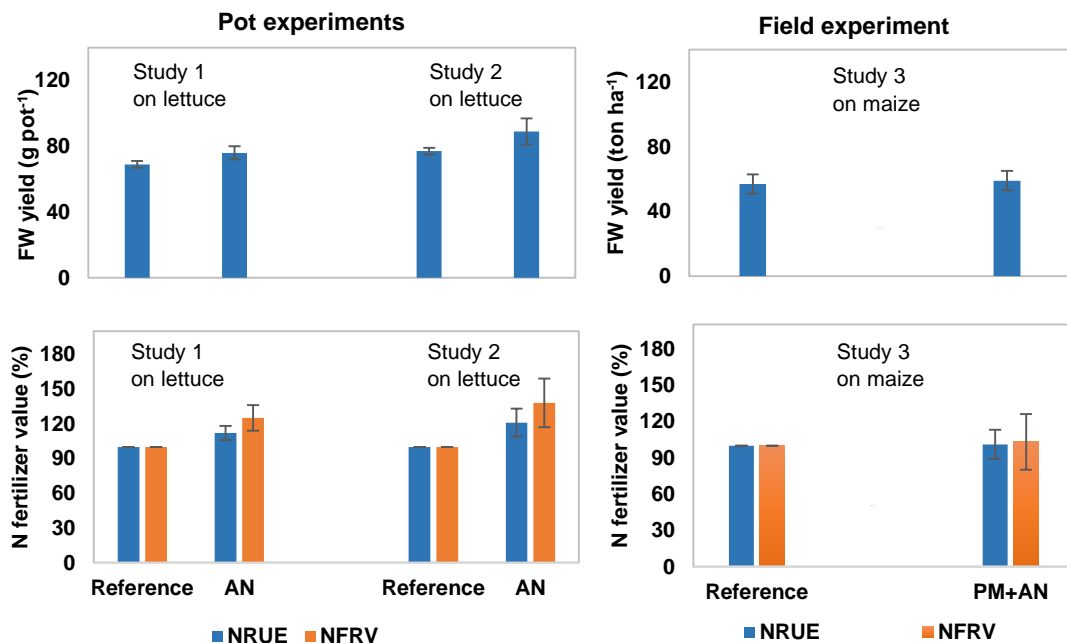
Figure 1. Effect of ammonium nitrate (AN) on fresh weight (FW) yield and its nitrogen (N) fertilizer value compared to conventional fertilisation regime in lettuce (Reference = calcium ammonium nitrate (CAN; 27%N) as synthetic N) and maize (Reference = pig manure (PM) + CAN). N replacement use efficiency (NRUE) does not account for the effect of unfertilised treatment, whereas N fertilizer replacement value (NFRV) takes into account the effect of unfertilised treatment. To determine NRUE and NFRV of ammonium nitrate, the reference treatment is considered to be 100% effective.
